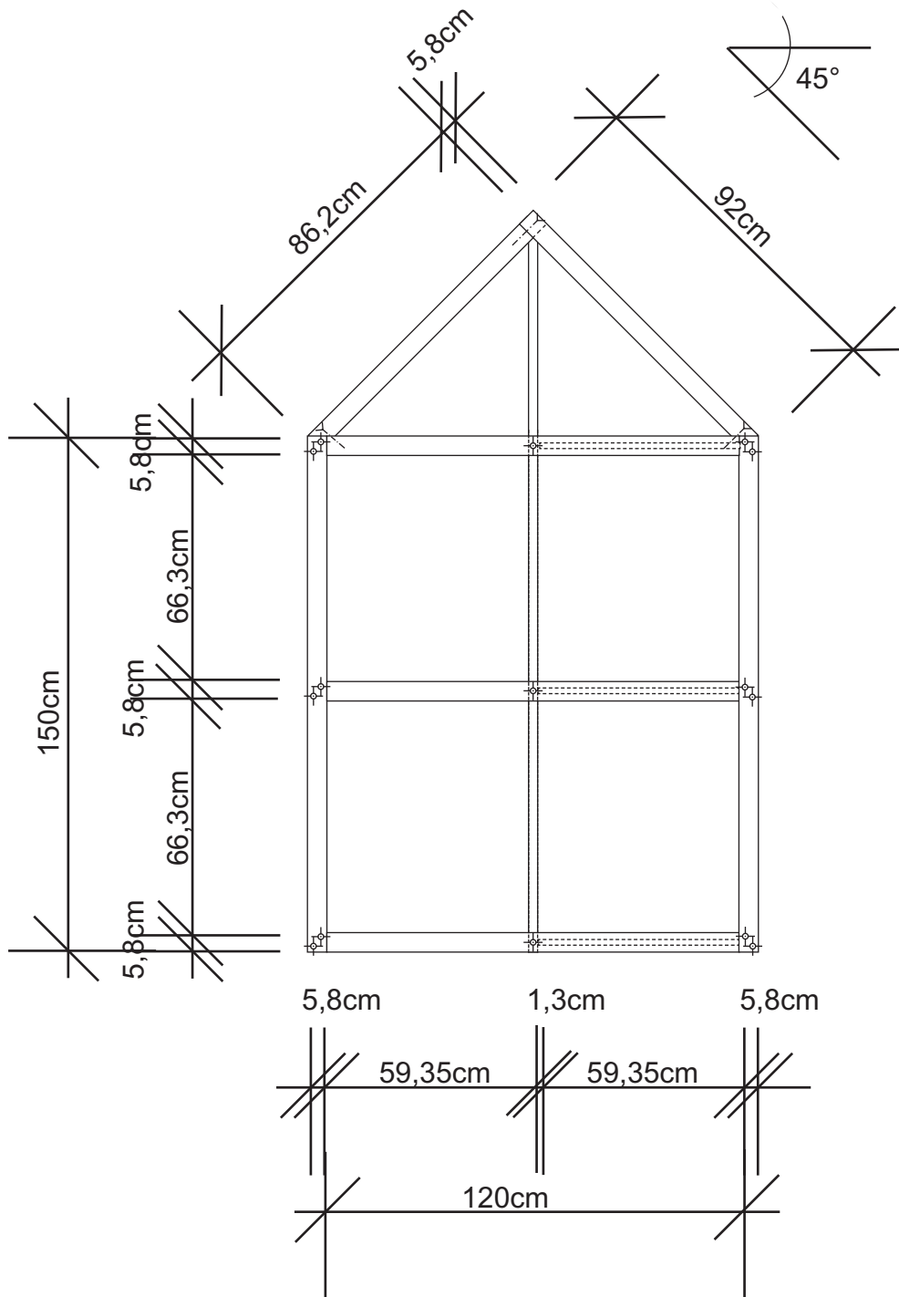
front view
